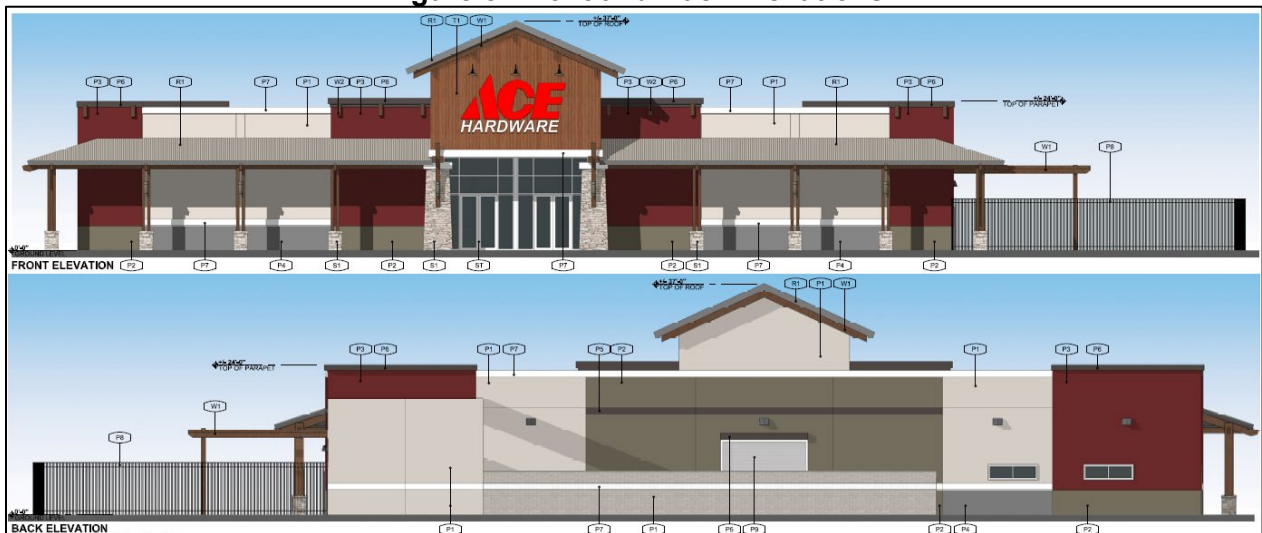
Figure 8: Front and Back Elevations
